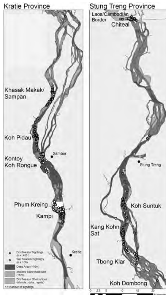
FIGURE 15.4 Distribution of Irrawaddy dolphins inhabiting the Mekong River, based on all dolphin sightings obtained between January 2001 and April 2005. Kratie province is shown on the left map and Stung Treng Province, which is further north (see Fig. 15.6) on the right map. Sightings are separated into dry season (red dots) and wet season (yellow dots). Map created by Erin LaBreaque and reproduced with her permission.
